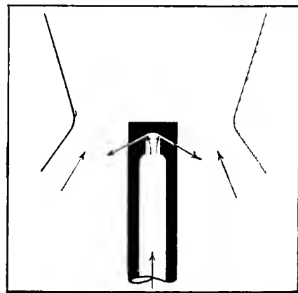
Fig. 2—Section through another type of jet in which the outlet is deflected downwards
